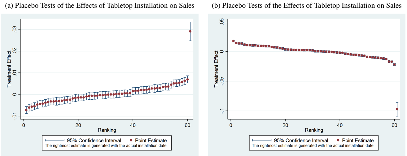
Figure 3: Placebo Tests
